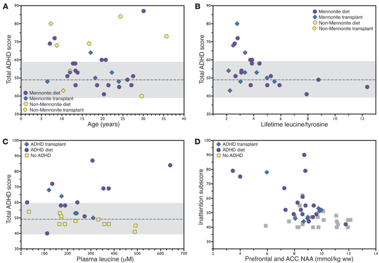
Figure 4 Clinical and neurochemical correlates of ADHD symptoms in MSUD patients. ADHD was inversely correlated to age (A) and directly related to the lifetime plasma leucine/tyrosine ratio (B). Plasma leucine at the time of the study does not correlate with ADHD symptoms scores. However, an interaction exists between plasma leucine and history of an ADHD diagnosis in predicting total ADHD ratings at the time of the study, such that in those patients who have ever had a diagnosis of ADHD, higher leucine levels corresponded with higher symptom ratings (C). Severity of inattention symptoms correlated with several metabolites, such as prefrontal and anterior cingulate (ACC) cortical NAA (D). Symbols: Mennonite MSUD diet (violet circles); Mennonite MSUD transplant (blue diamonds); non-Mennonite MSUD diet (yellow circles); non-Mennonite transplant (yellow diamonds); no ADHD (yellow squares); control subjects (gray shaded areas [mean ± SD] or gray squares).
