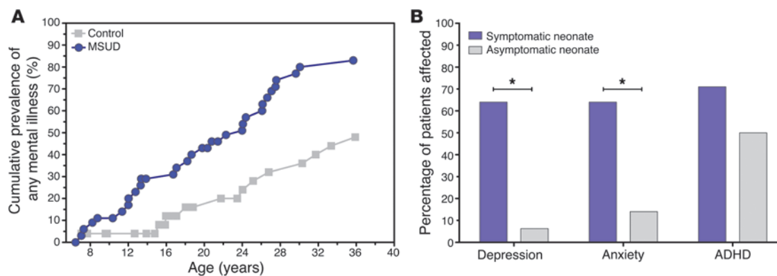
Figure 2 Cumulative prevalence and neonatal risks associated with neuropsychiatric outcome in classical MSUD patients. The cumulative lifetime incidence of mental illness (depression, anxiety disorders, ADHD) among all MSUD patients reached 83% by age 36 (A). Neonatal encephalopathy was a strong predictor of mood disorders, but not mental retardation or ADHD, later in life (B). * P < 0.05 .
