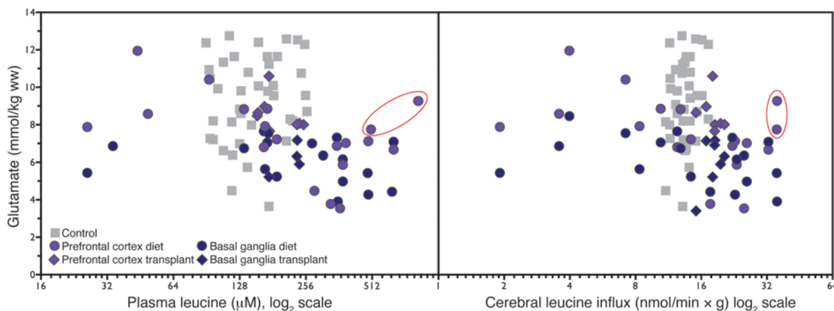
Figure 1 Glutamate (in mmol/kg wet weight, ww) in the prefrontal and anterior cingulate cortices (violet) and basal ganglia (blue) region inversely correlated with ambient plasma leucine (left panel) and the calculated cerebral leucine influx (right panel) in MSUD patients on diet (circles) or after liver transplantation (diamonds). Control subjects are represented as gray squares. The 2 MSUD diet patients who demonstrate relatively higher cortical glutamate levels despite having the highest estimated leucine influx are brothers (circled in red).
